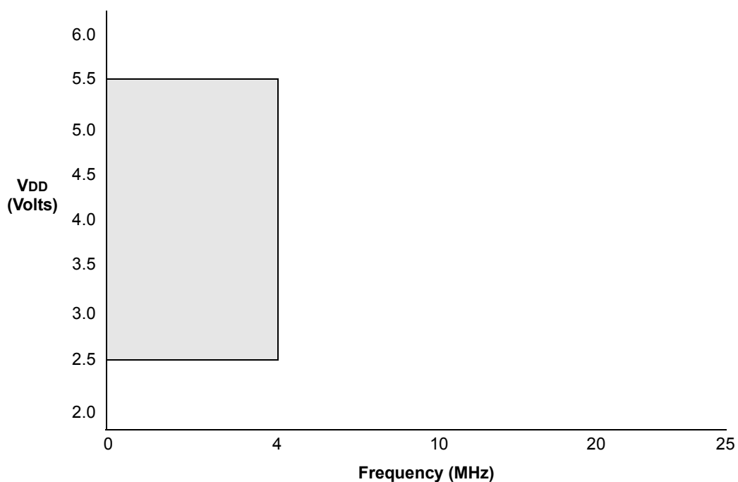
FIGURE 2: PIC16LC505 VOLTAGE-FREQUENCY GRAPH, 0^{\circ}\text{C} \leq T_A \leq +70^{\circ}\text{C}
