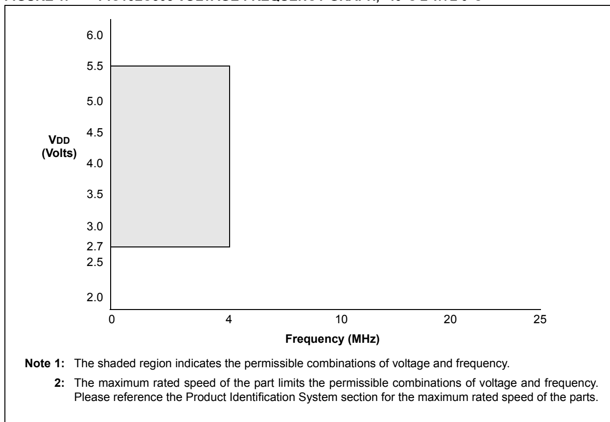
FIGURE 1: PIC16C505 VOLTAGE-FREQUENCY GRAPH, -40^{\circ}\text{C} \leq T_A \leq 0^{\circ}\text{C}
